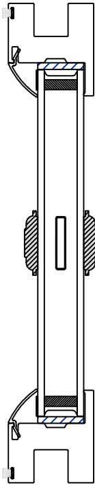
SDL Sculptured Simulated Divided Lite
