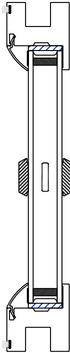
SDL 1" Flat Simulated Divided Lite
