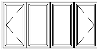
I 750 LHC-FC-FC-RHC
