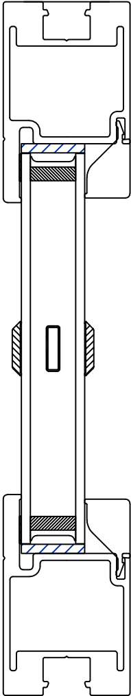
SDL Flat Simulated Divided Lite
