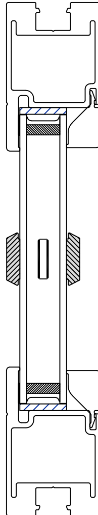
SDL 1" Flat Simulated Divided Lite
