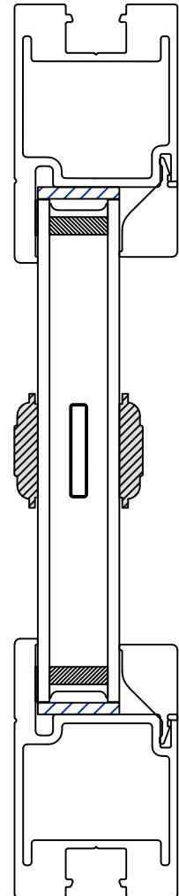
SDL Sculptured Simulated Divided Lite
