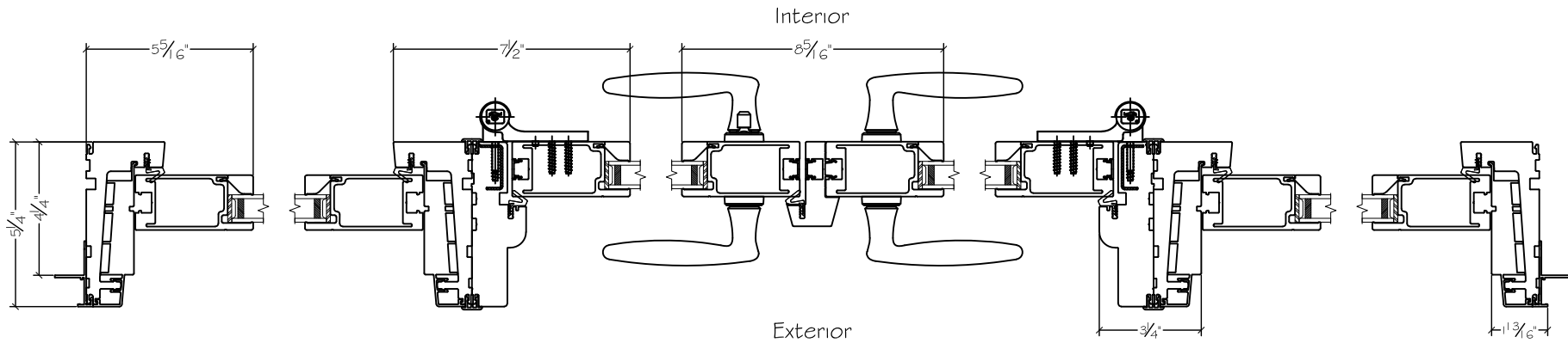
3750 Swing Door 1-inch Nail-fin Configuration
